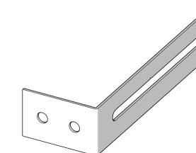
Floating Wall Clip (Long) G25FWCL
