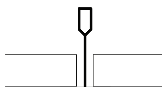
24mm Grid (Square Edge)
