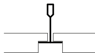
24mm Grid (Rebated Edge)
